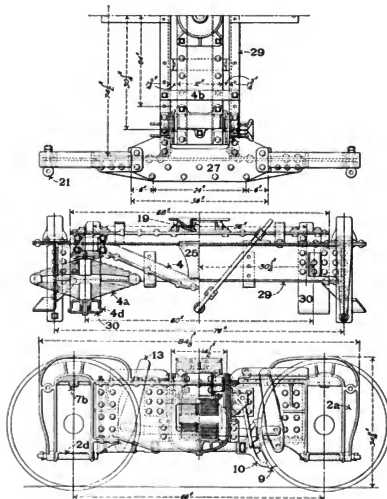
Figs. 4352-4354. Pedestal Tender Truck. Standard Steel Car Co.
